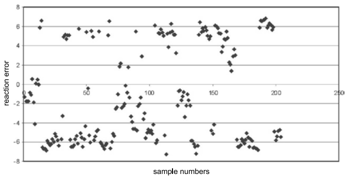
Fig. 4. Ionic balance reaction error
