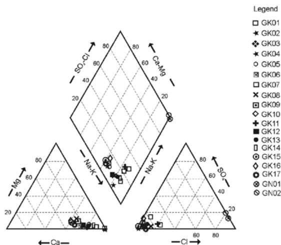
Fig. 6. Chemical analysis of water of the study area plotted on the Piper diagram
